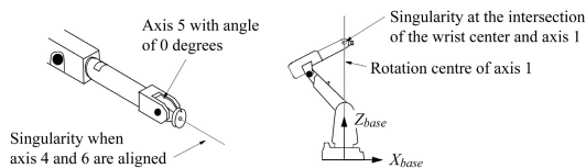
Fig. 2. Wrist singularities occur when axis 5 is 0 degrees (left). An arm singularity where the wrist center and axis 1 intersect (right). [3]
