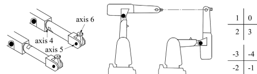
Fig. 3. Two different wrist (left) and arm configurations to attain the same position and orientation (center). Quarter revolutions for the joint angles as final target configuration (right). [3]
